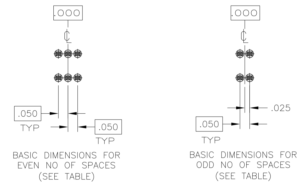
DETAIL R
